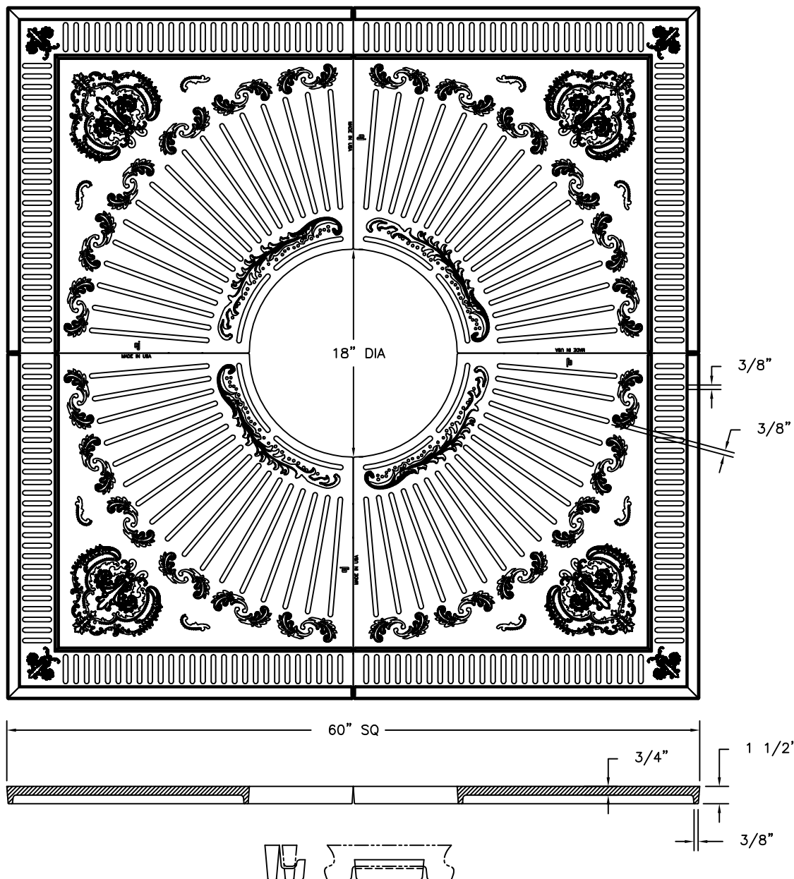
INTERLOCK ASSEMBLY DETAIL
